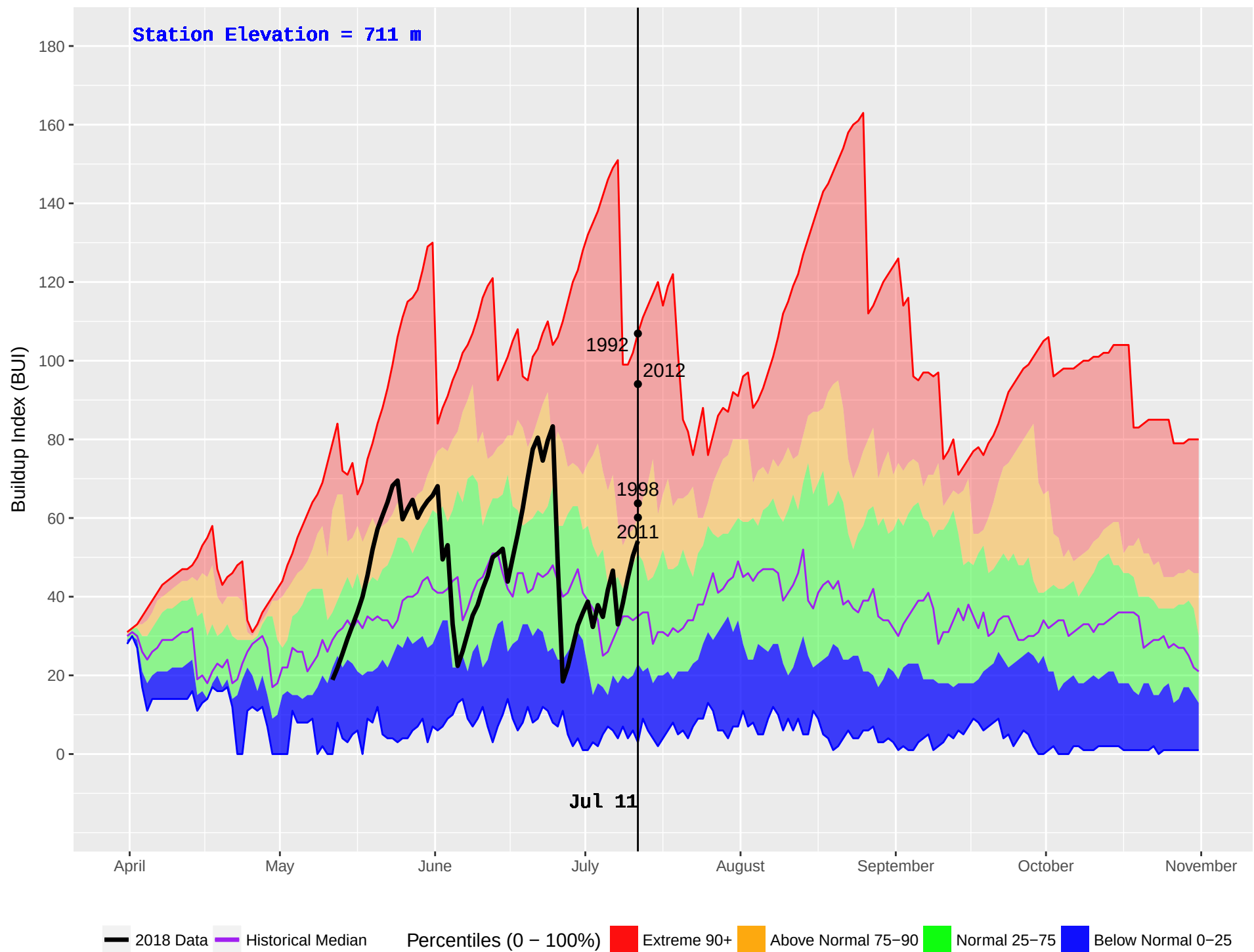
TOAD RIVER (126) : Historical (1981–2016) and Current (2018) Noon Buildup Index (BUI)
